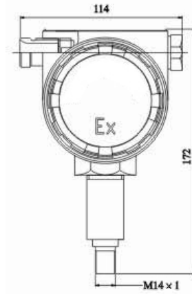
4-20mA & Pulse Transmitter-No Display Ex-Proof
